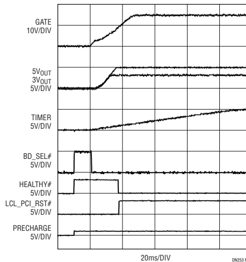
Figure 2. Normal Power-Up Sequence
